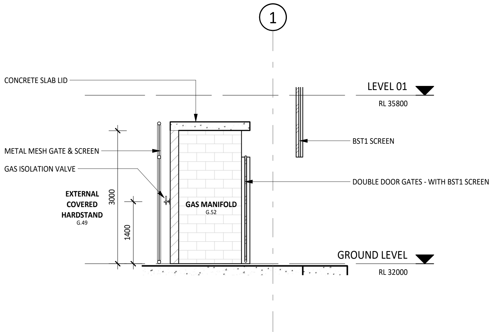
2 GAS MANIFOLD SECTION 60-028 1 : 50
